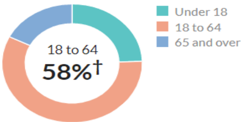
Population by age category
